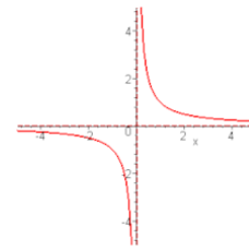
Hyperbel
