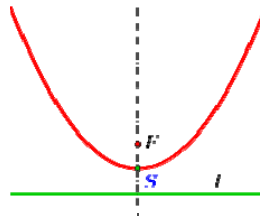
Parabel
