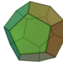
Dodekaeder (Äther)
